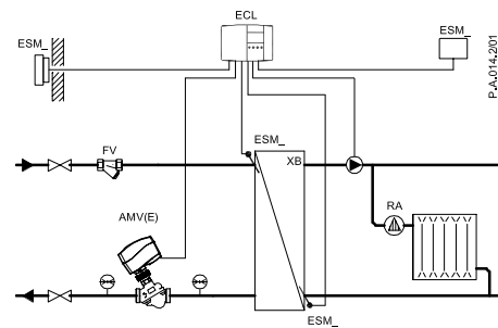
AMV(E) 130(H)/140(H) + AHQM
